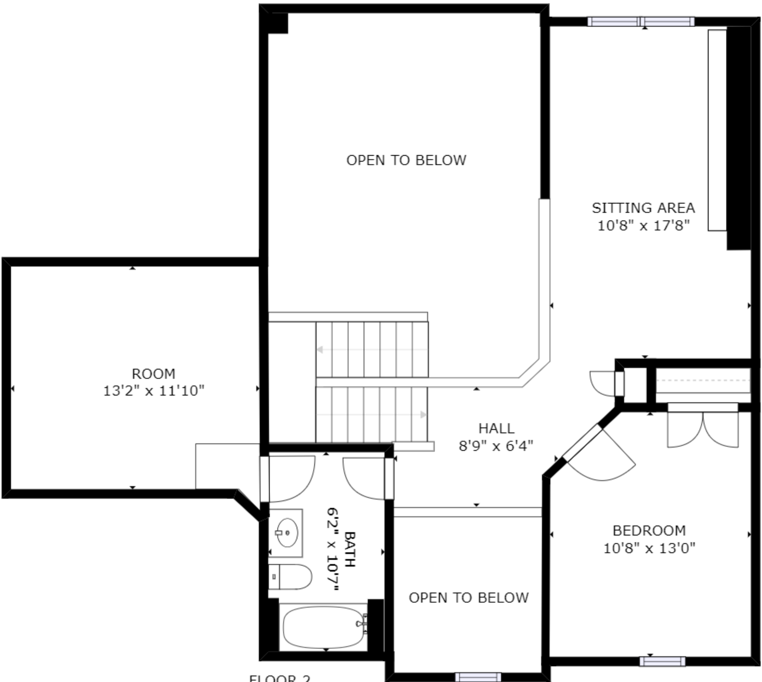
FLOOR 2
